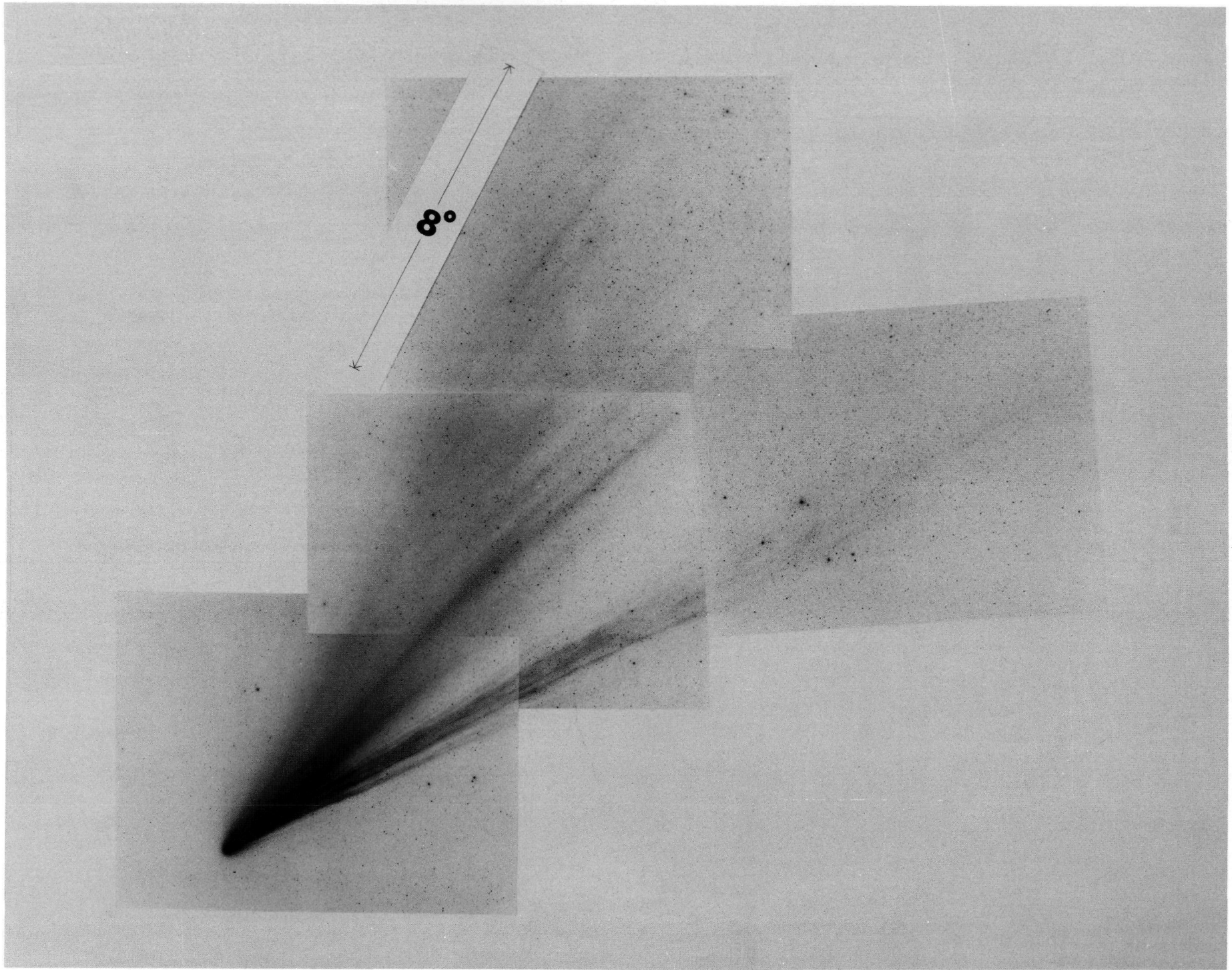
Figure 9. Mosaic of JOCR photographs showing comet West on March 9, 1976.
